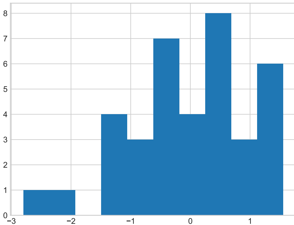
Standardized deviance residuals
